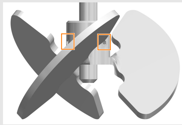
Pitched blade impeller (version for cell cultures)
