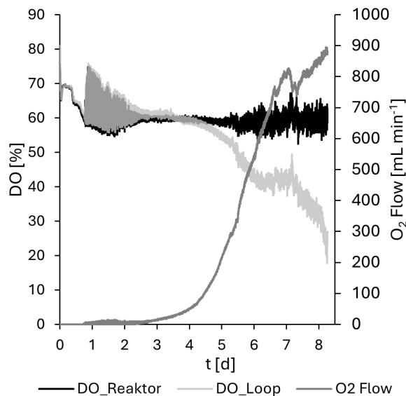
Figure 7. Dissolved oxygen (DO) in the bioreactor, recirculation loop, and O 2 flow rate during cultivation 2.
